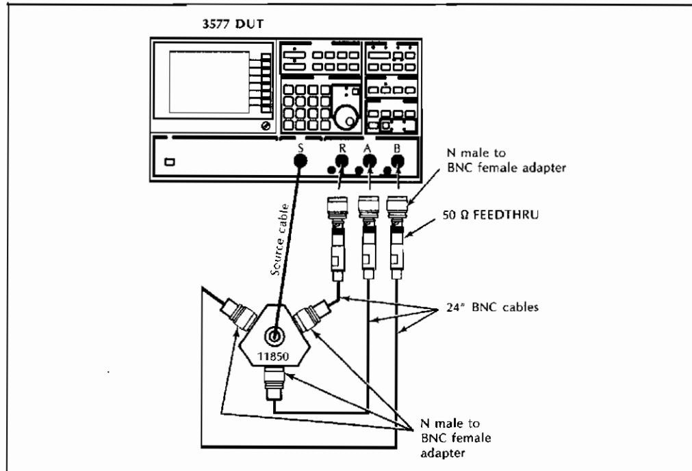
Figure 3-14 Ratio Test Set-Up (1 M \Omega )
