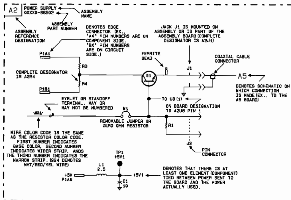
Figure 8-1. Reference Designations
