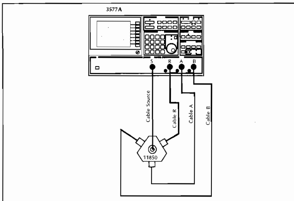
Figure 3-13 Ratio Test Set-Up (50 \Omega )
